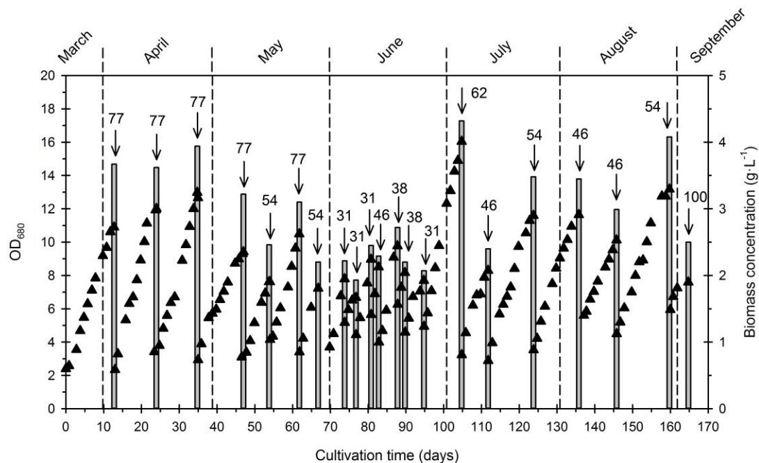
Fig. 5. Cultivation of N. atomus in the floating 65-L HBR during outdoor semi-continuous operation in central Florida. Daily growth as monitored by OD_{680} ( \blacktriangle ); arrows and their adjacent labels mark culture harvesting and % of total reactor volume harvested, respectively; gray bars show the biomass concentration at harvest.
