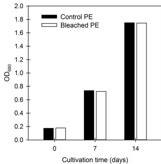
Fig. 2. Cultivation of N. atomus in the presence of original PE (control) and bleached PE pieces to account for any adverse effect of PE bleaching on cell growth.
