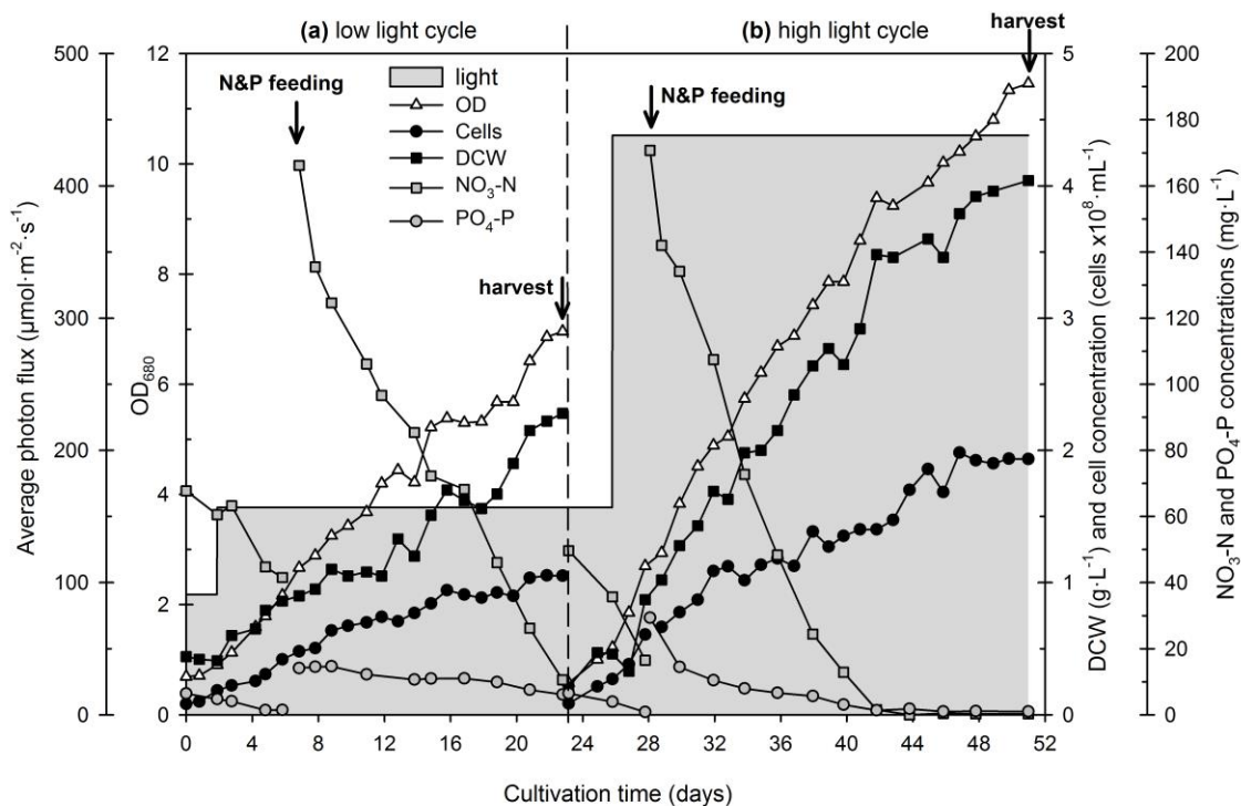
Fig. 3. Growth and nutrient consumption of N. atomus during the two cultivation cycles, 0-23 rd day and 23 rd -52 nd day, in the floating HBR under two artificial illumination levels of (a) 11.3 klux and (b) 31.1 klux. After the 1 st cycle (growth in low light) 90% (v/v) of the culture was harvested and the residual 10% (v/v) was used as inoculum for the 2 nd cycle (growth in high light). The arrows mark either nutrient (nitrate and phosphate) feeding or culture harvesting.
